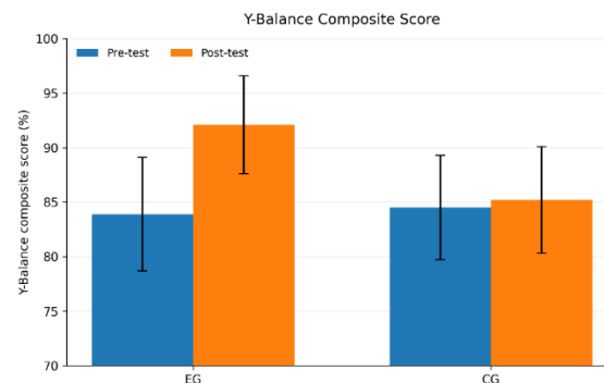
Fig. 2. Pre- and post-test Y-Balance composite scores (%) in the experimental (EG) and control (CG) groups. Data are presented as mean \pm SD.
