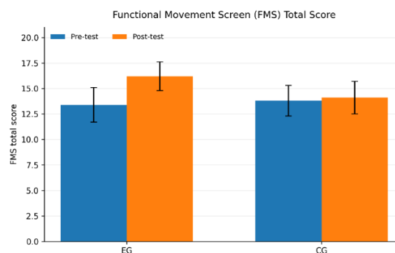
Fig. 3. Pre- and post-test Functional Movement Screen (FMS) total scores in the experimental (EG) and control (CG) groups. Data are presented as mean \pm SD.
