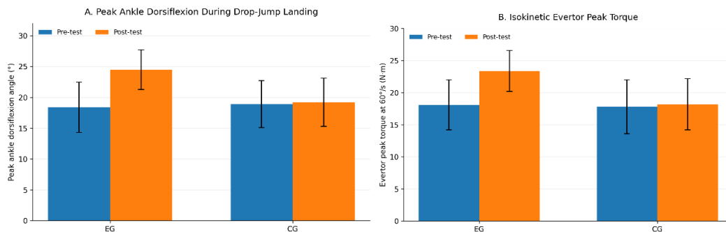
Fig. 1. Pre- and post-test biomechanical outcomes in the experimental (EG) and control (CG) groups: (A) peak ankle dorsiflexion angle (°); (B) isokinetic evtor peak torque at 60°/s (N·m). Data are presented as mean \pm SD.
